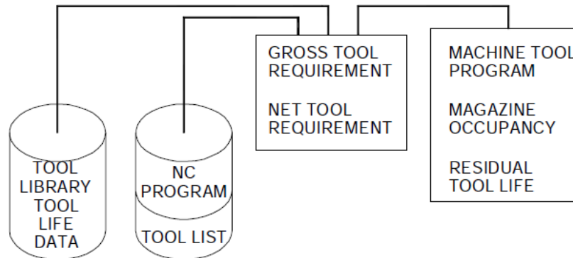
Fig. 36 Data Requirements
