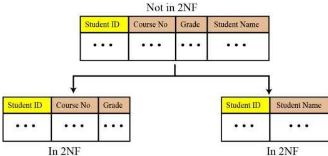
Fig 129 An example of 2NF
