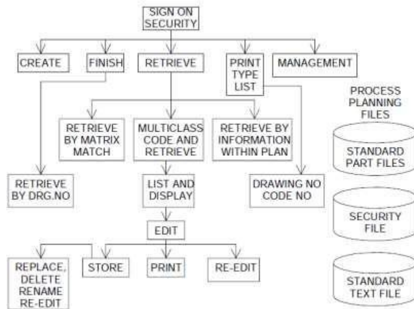
Fig. 16 MULTICAPP System
