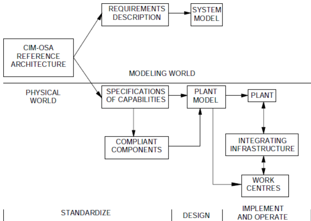
Fig. 78 Operating Environment to Apply CIM-OSA Model
