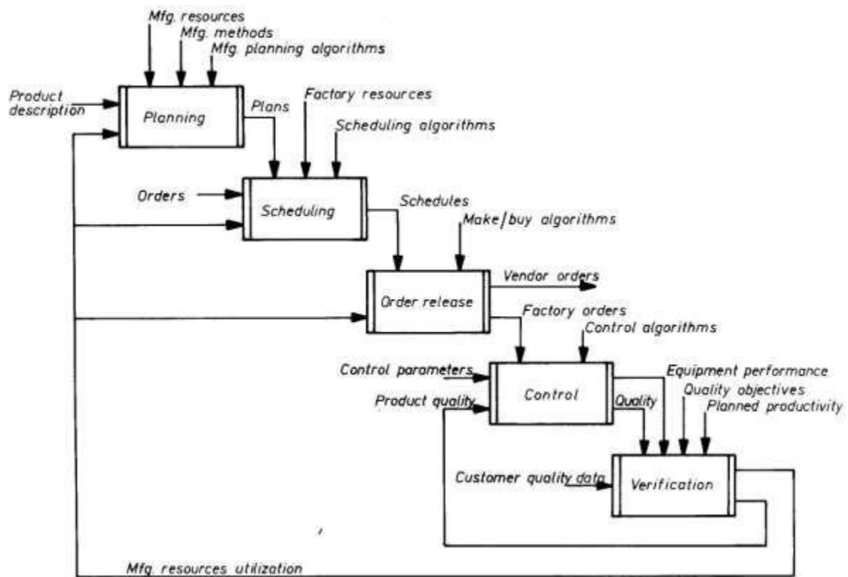
Fig. 48 Control Loop of a Manufacturing System
